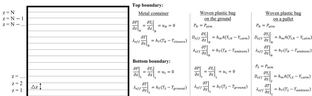
Figure 2. Discretization and the boundary conditions.
