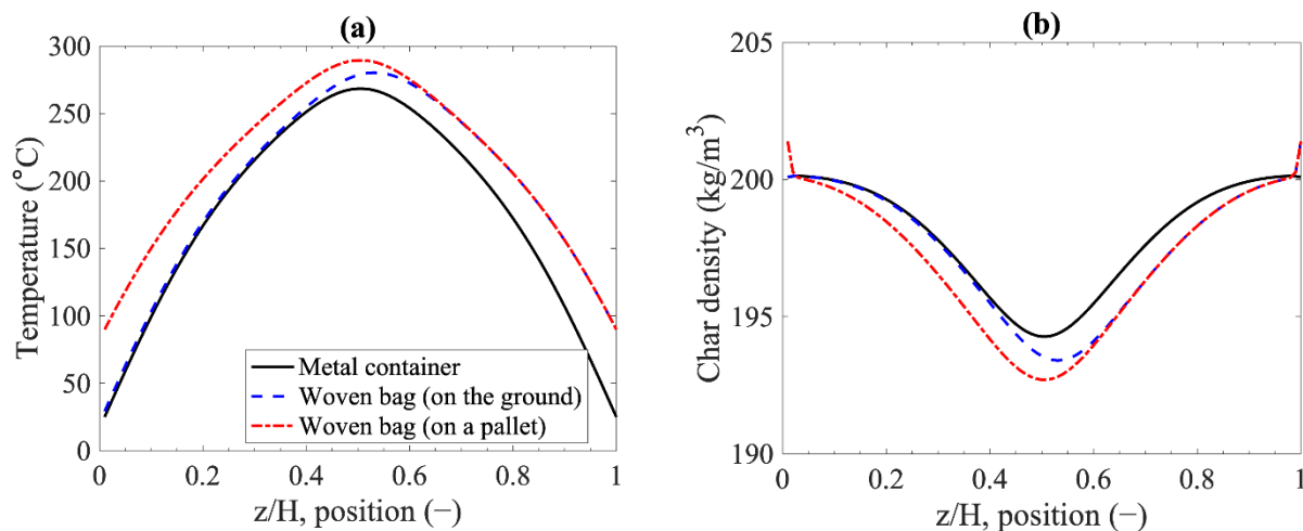
Figure 10. Local profiles inside the storage container after 12 h (storage condition: T_0 = 210\text{ }^{\circ}\text{C} , T_{\text{ambient}} = 25\text{ }^{\circ}\text{C} , \rho_{c,0} = 200\text{ kg m}^{-3} , and H_{\text{container}} = 1\text{ m} ): (a) char temperature; (b) char density.
