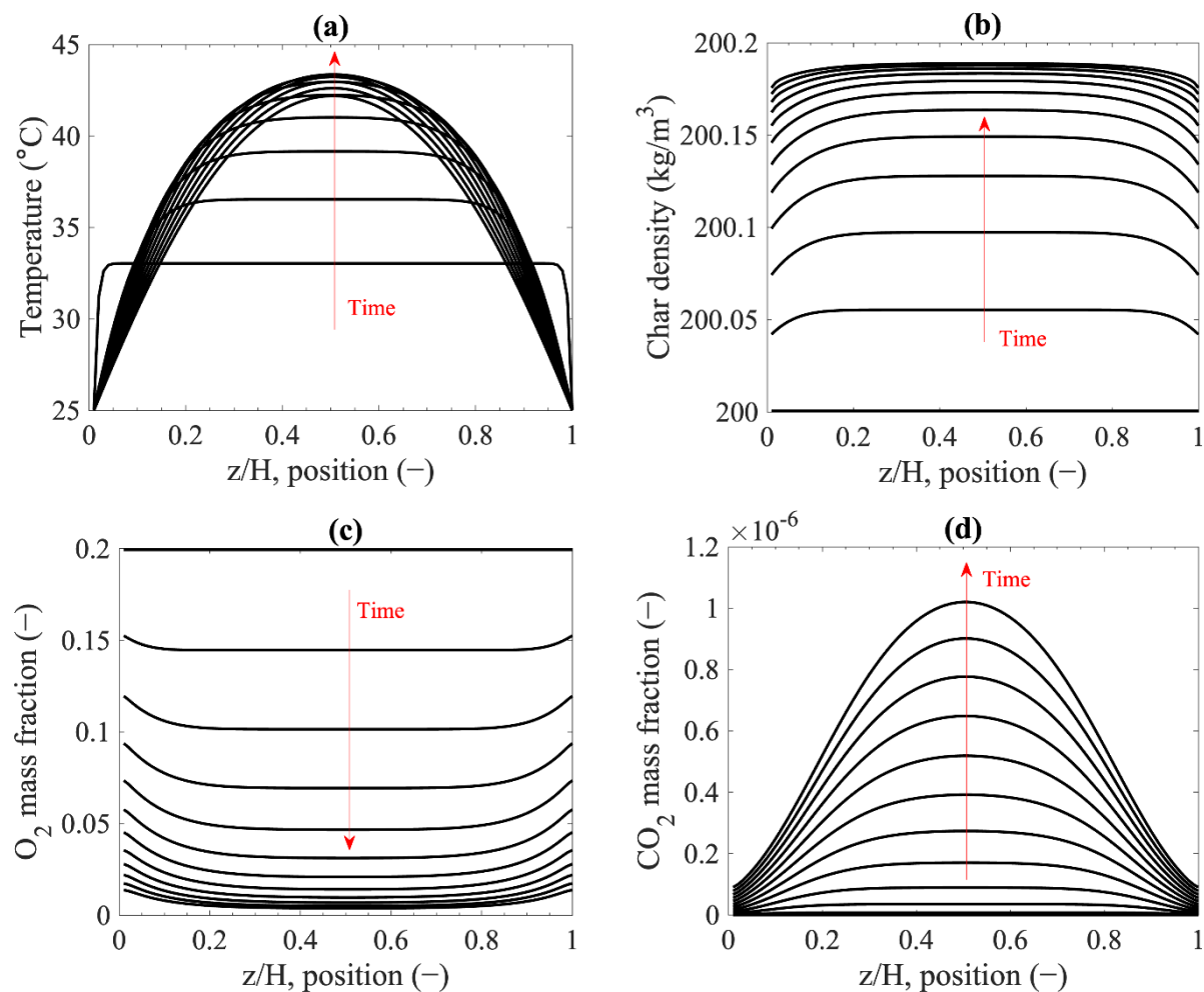
Figure 5. Evolution of local properties over time with the interval of 100 min (Conditions: T_0 = 33\text{ }^{\circ}\text{C} , T_{\text{ambient}} = 25\text{ }^{\circ}\text{C} , \rho_{c,0} = 200\text{ kg m}^{-3} , and H_{\text{container}} = 1\text{ m} ): (a) Local temperature; (b) char density; (c) \text{O}_2 mass fraction; (d) \text{CO}_2 mass fraction.
