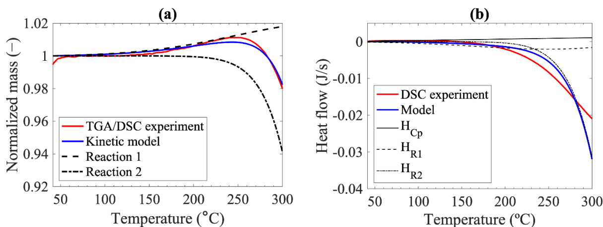
Figure 3. TGA-DSC result in comparison with the models for: (a) mass; and (b) heat.
