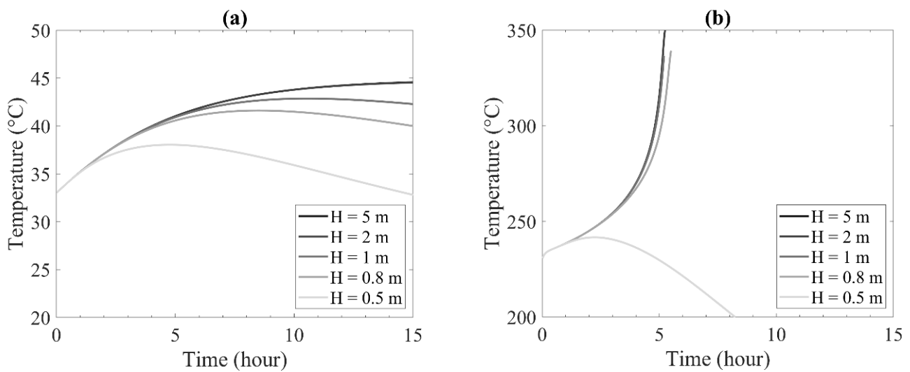
Figure 7. Effect of container size on the temperature at the center of the container with the conditions of T_{\text{ambient}} = 25\text{ °C} , \rho_{c,0} = 200\text{ kg m}^{-3} : (a) initial char temperatures of 33 °C; (b) initial char temperatures of 230 °C.
