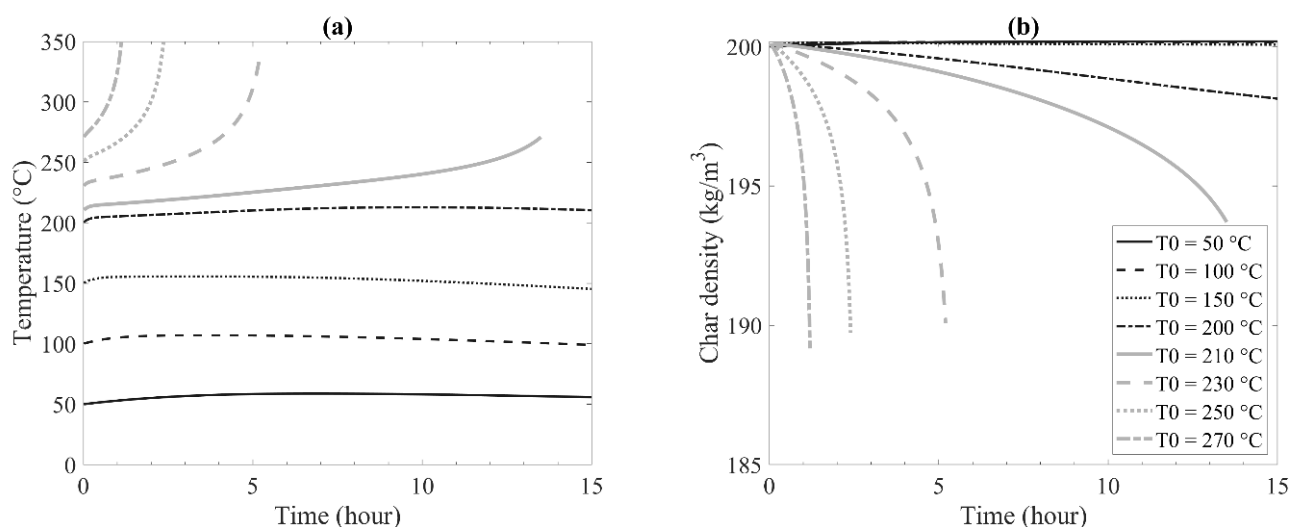
Figure 9. Effects of char initial temperature with the storage condition of T_{\text{ambient}} = 25 °C, \rho_{c,0} = 200 kg m -3 , and H_{\text{container}} = 1 m: (a) on thermal runaway represented by the average char temperature; (b) on average char density.
